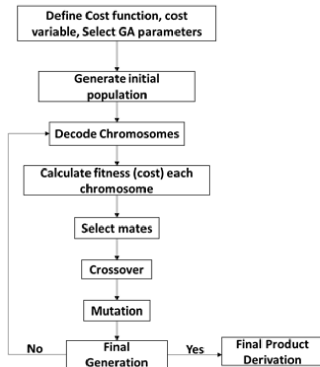
Figure 2. Genetic algorithm process.
